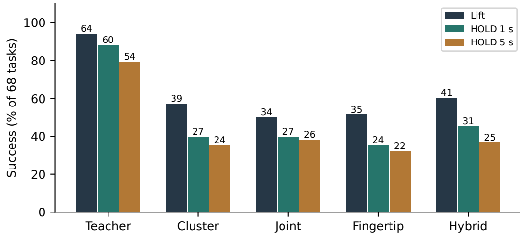
(a) Common held-out evaluation
